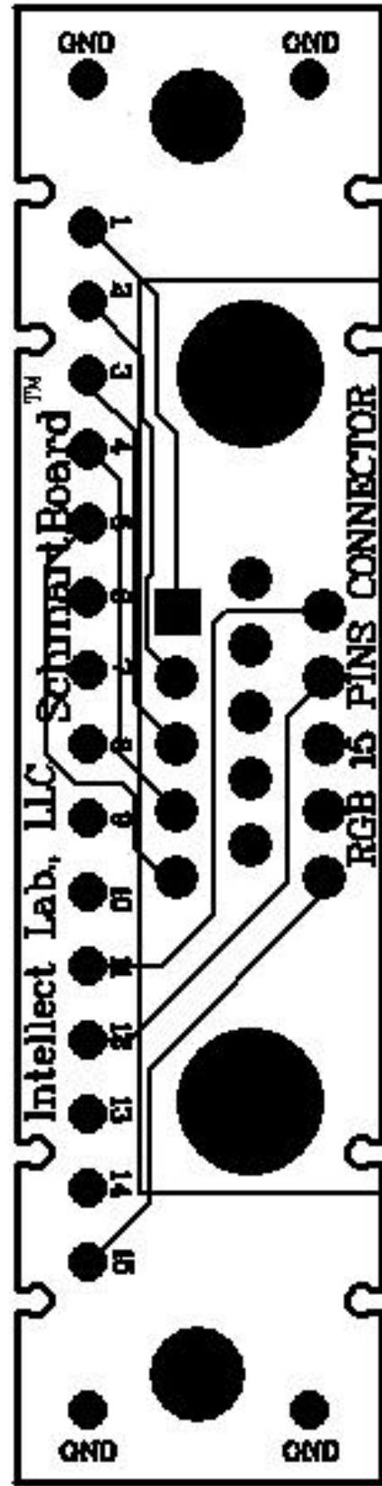
RGB CONNECTOR (201-0106-01)
