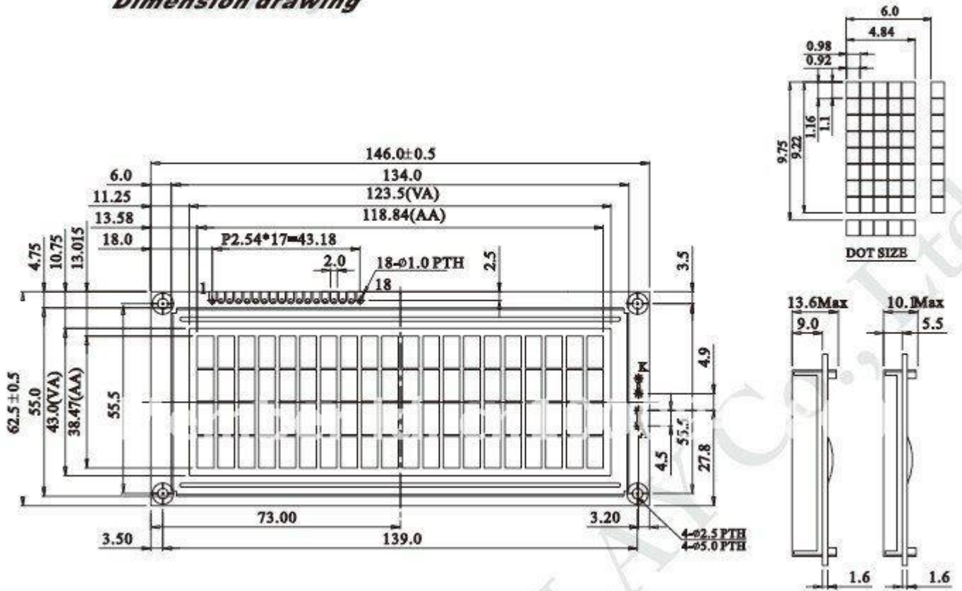
Dimension drawing
