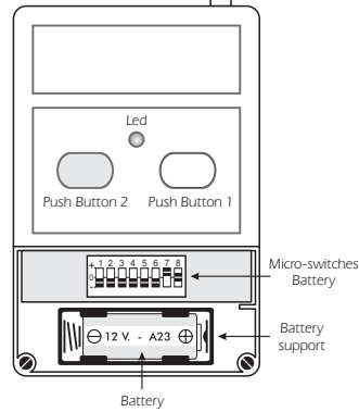
Enclosure opened, with front cover.
